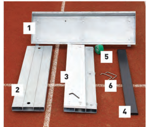
Foundation Equipment
